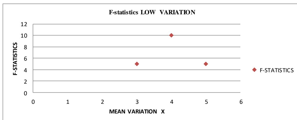
Graph No. 5 : Based on F-statistics with closure mean variation
