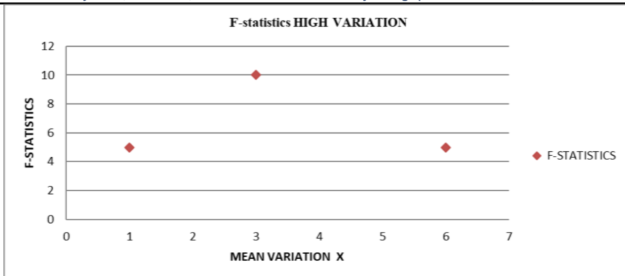
Graph No 3 :Analysis of variance can be obtained for design purposes ,Based on F-statistics with larger mean variation
