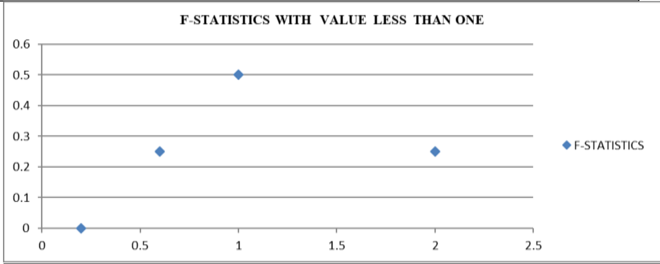
Graph No. 1 F-statistics Value less than 1
