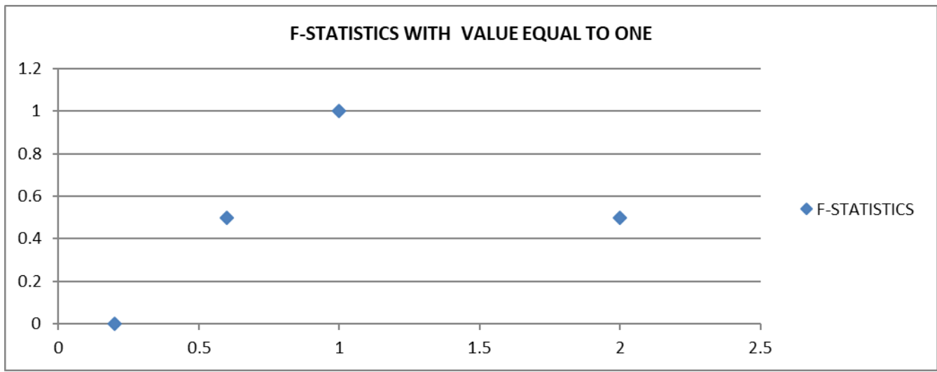
Graph No.2 F-statistics Value equal to 1
