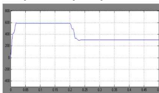
Figure5. RMS Load voltage with sag conditions
