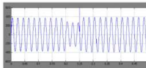
Figure 17. Load voltage with sag conditions
