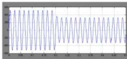
Figure 12. Load voltage with sag conditions
