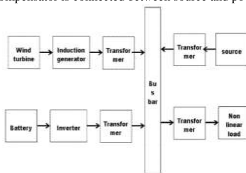
Figure 2. Block Diagram
