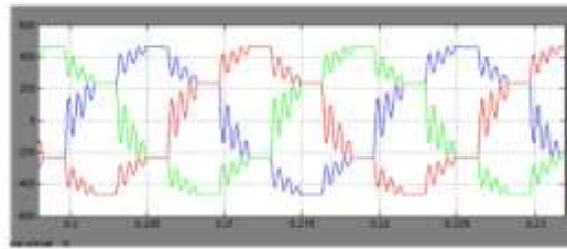
Figure 15.Generator side voltage
