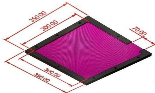
Figure 5.2 die design
