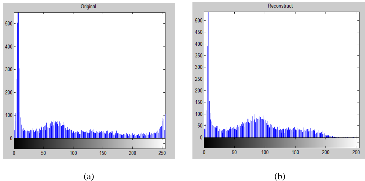
Figure 12: Histogram of (a) original data/image (b) reconstruct data/image
