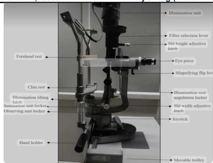
Figure1. 5: Slit Lamp Microscope
