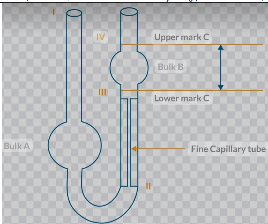
Figure 4.8: OSTWALD VISCOMETER
